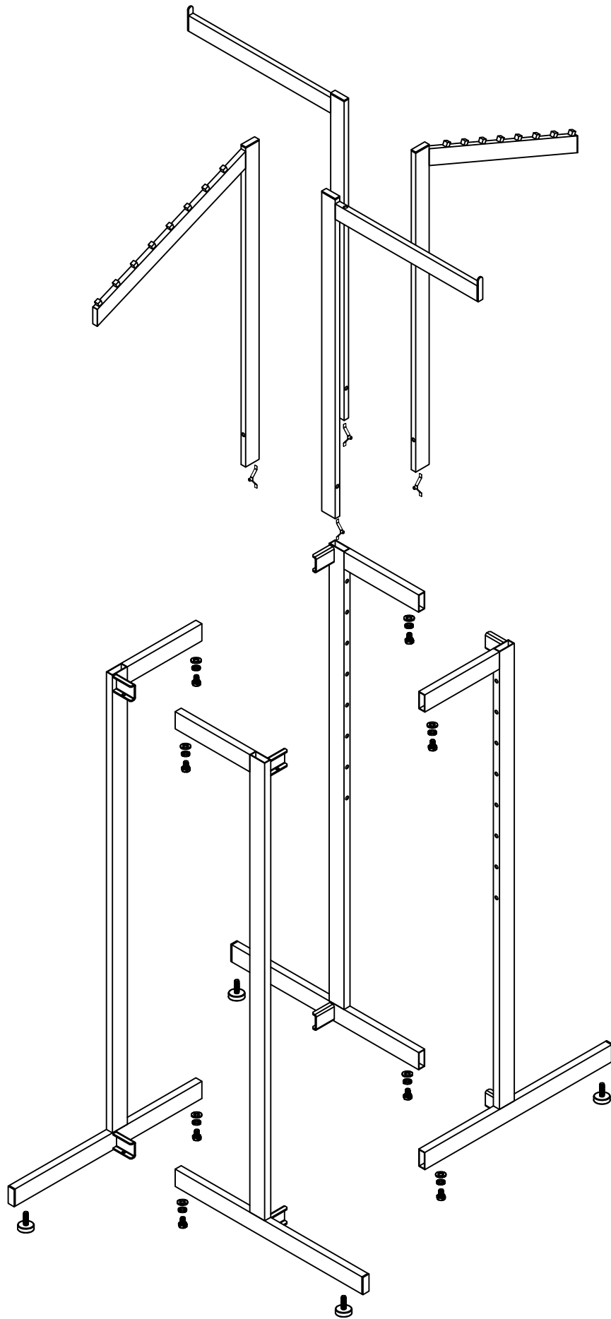
EXPLODED-ASSEMBLY RR422
